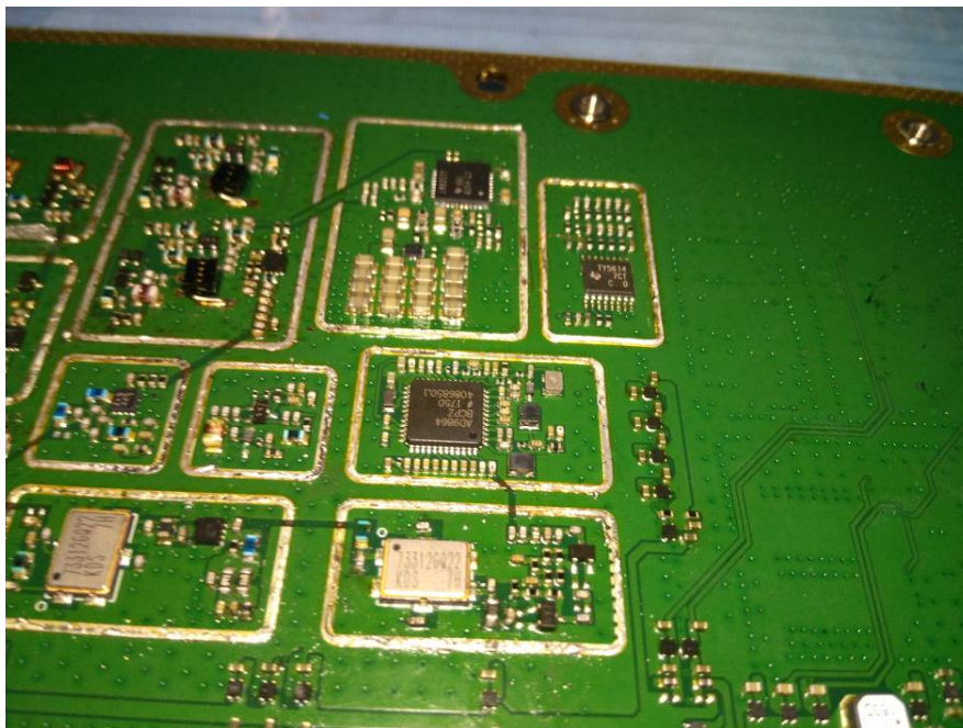
EUT – IC 6 View
