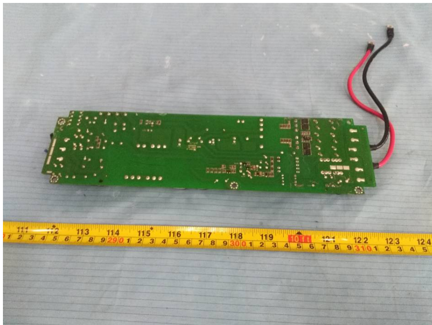
EUT – Power Supply Main Board Top View
