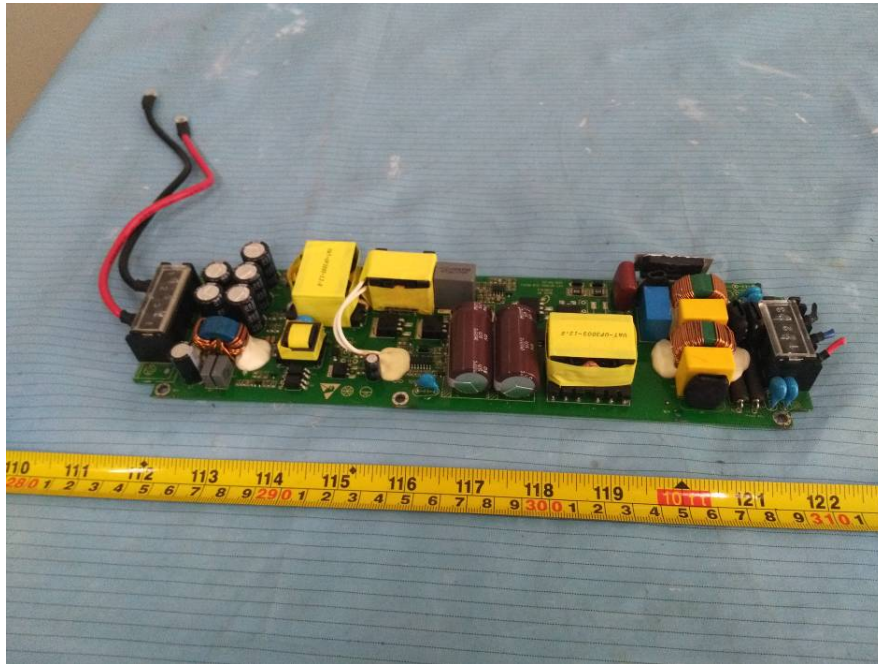
EUT – Power Supply Main Board Bottom View
