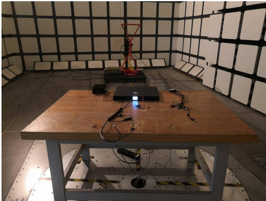
AC Power: Radiated Emissions – Front View (Below 1 GHz)
