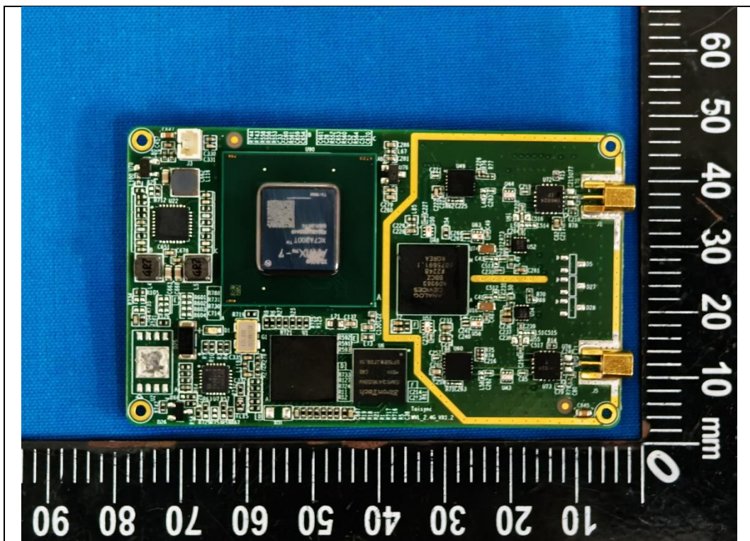
RF Chip
