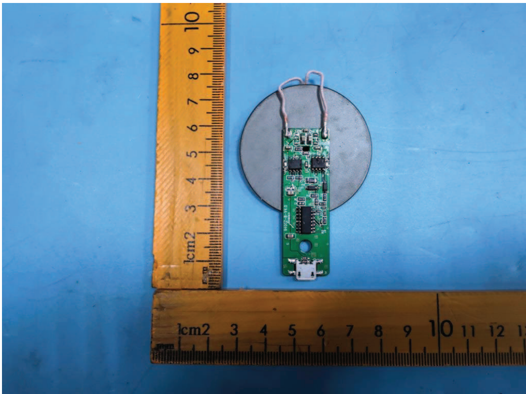
Fig. 5: Charging pad internal view
