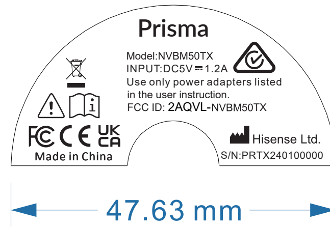
TX Rating label
