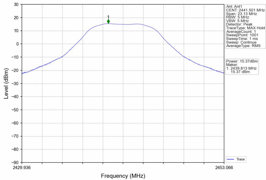
FHSS Middle Channel
