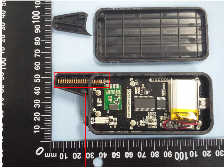
433MHz Antenna
