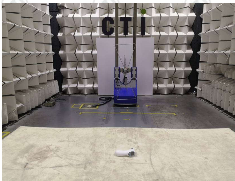
Radiated spurious emission Test Setup-2(Below 1GHz)
