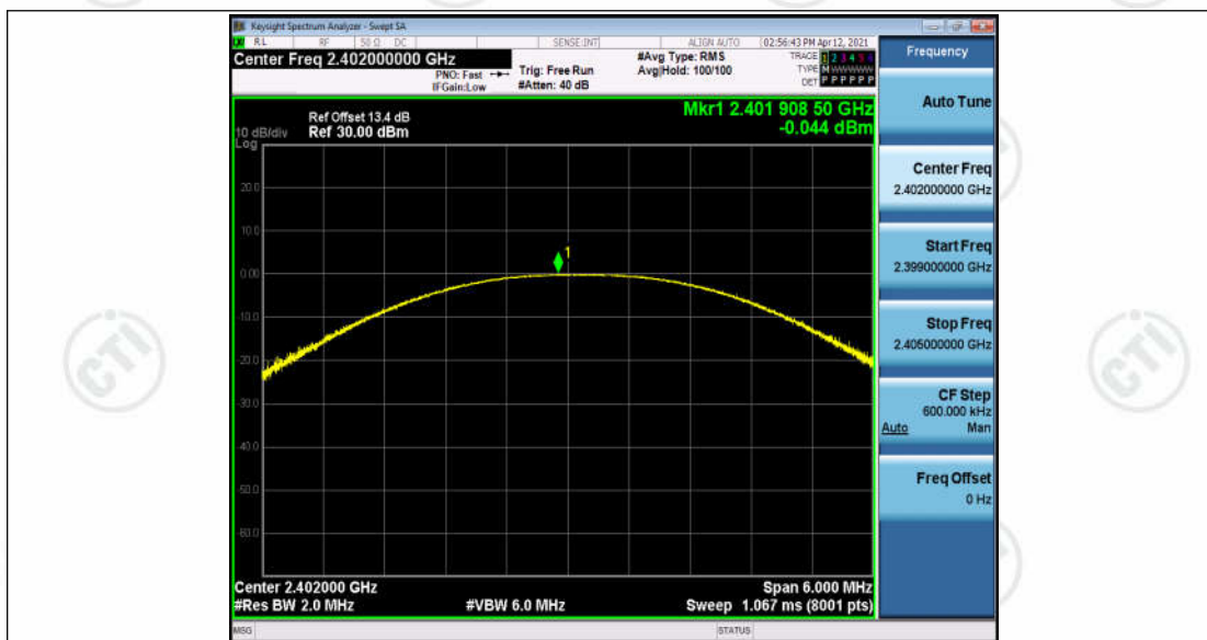
BLE_1M_Ant1_2402
