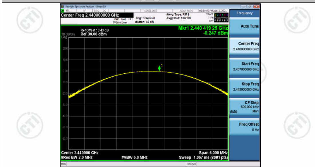
BLE_1M_Ant1_2440
