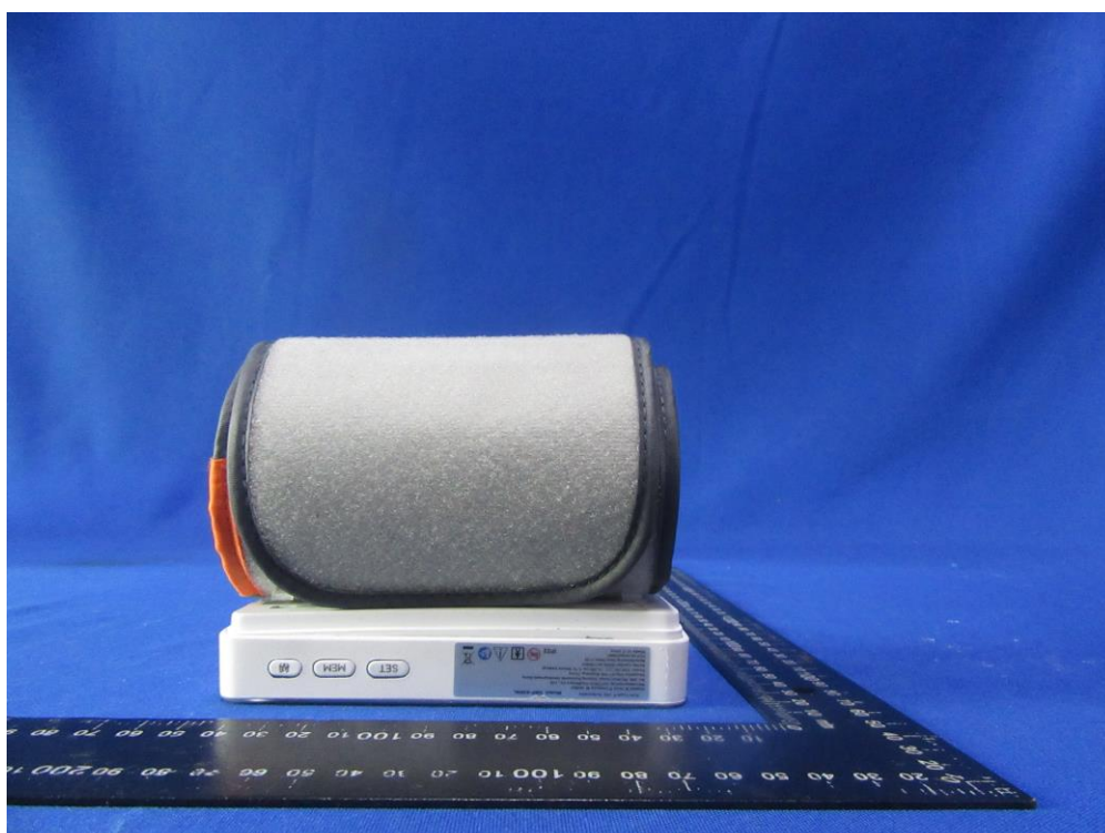
(4) EUT Photo - DBP-63D9L
