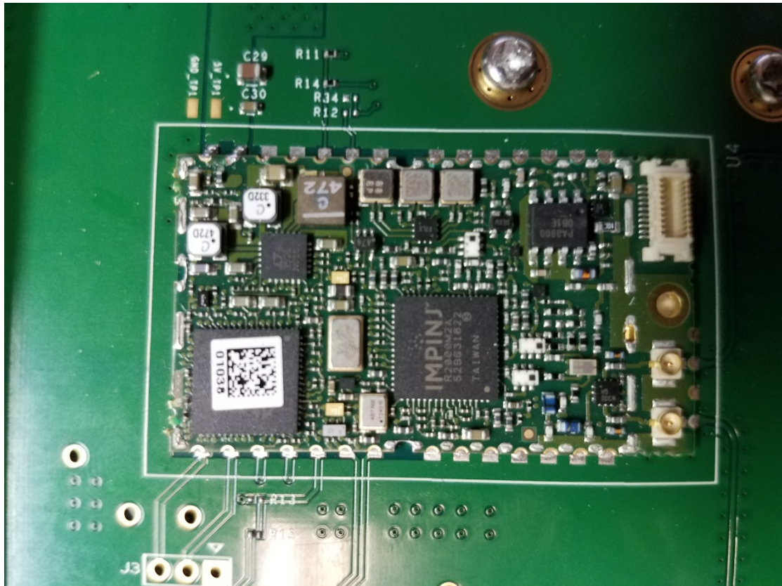
RFID Module with Cover Removed
