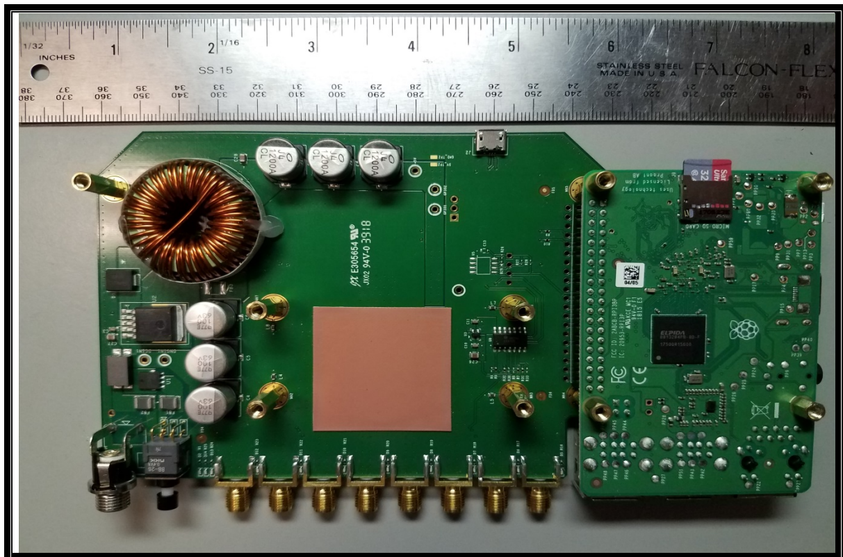
The rear PCB photo
