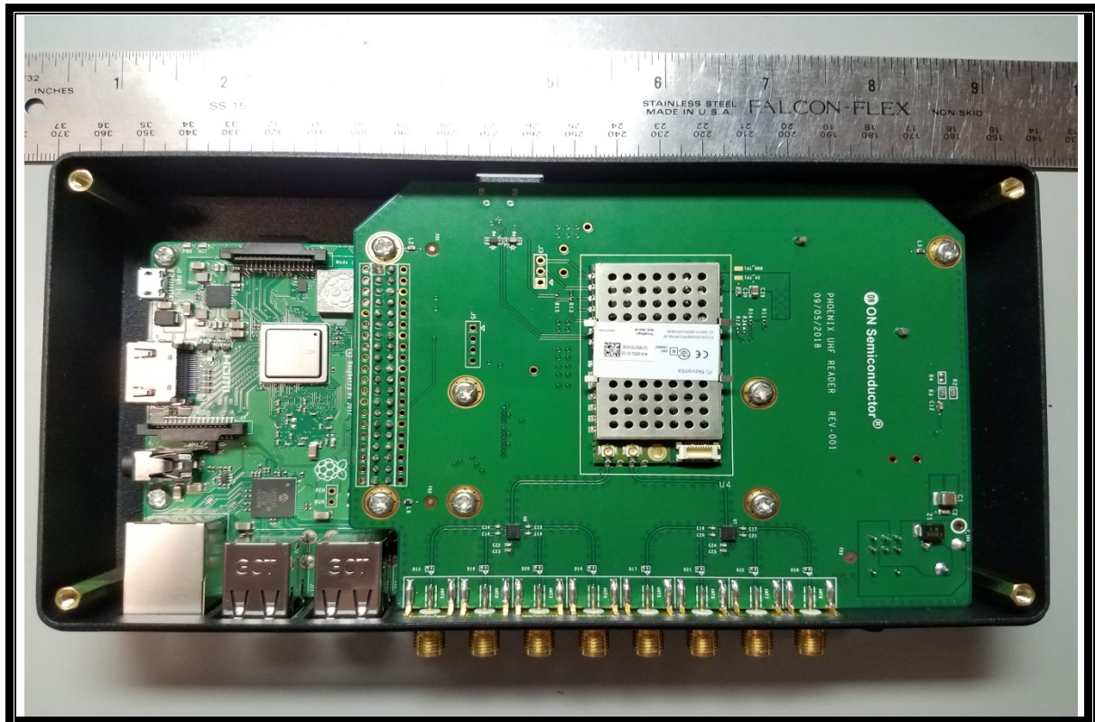
The equipment internal photo
