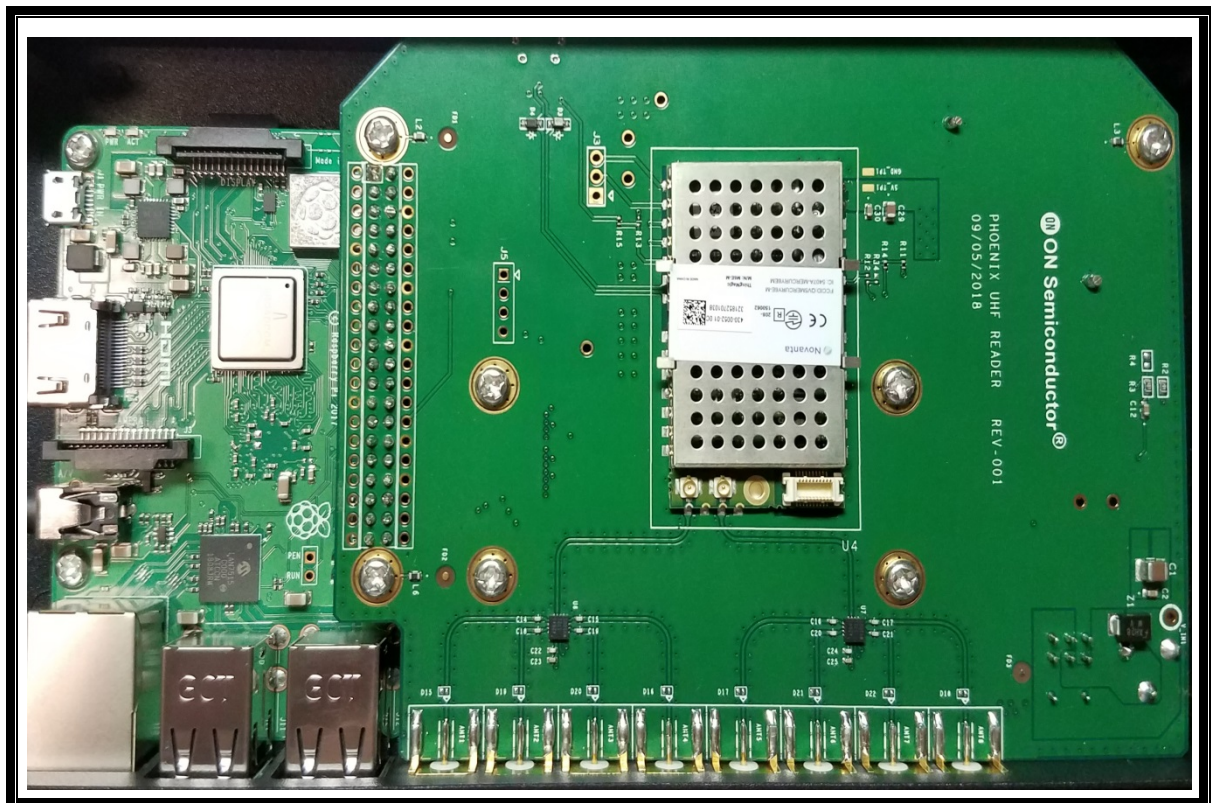
The front PCB photo
