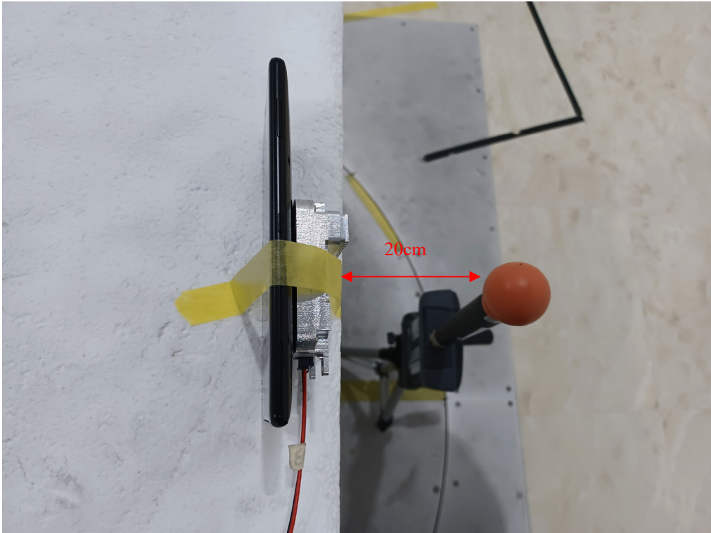
Bottom (20cm)
