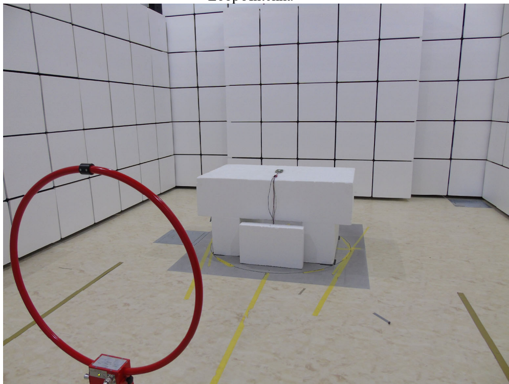
Loop Antenna
