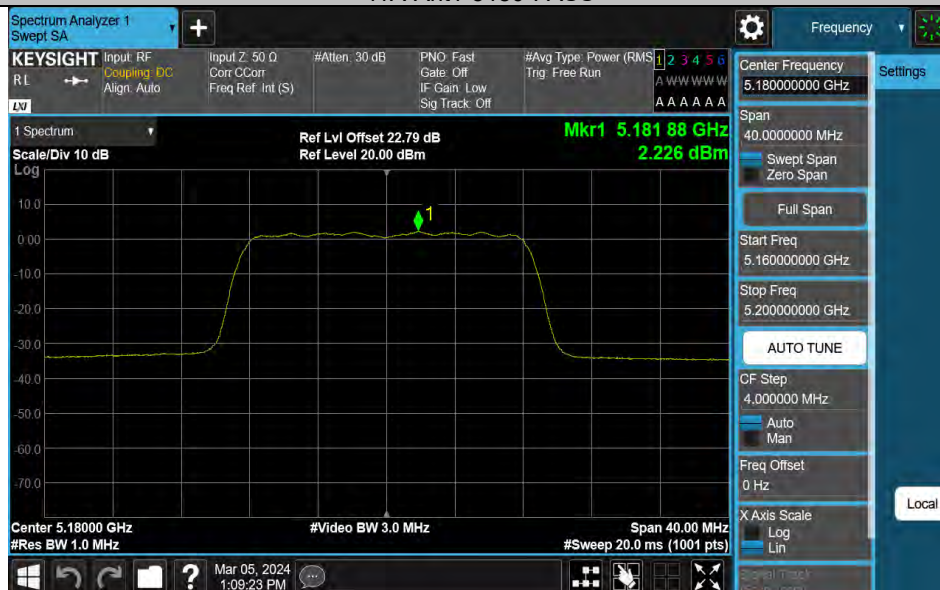
11A-Ant2-5180-PASS
