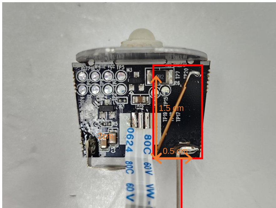
Wire Antenna
