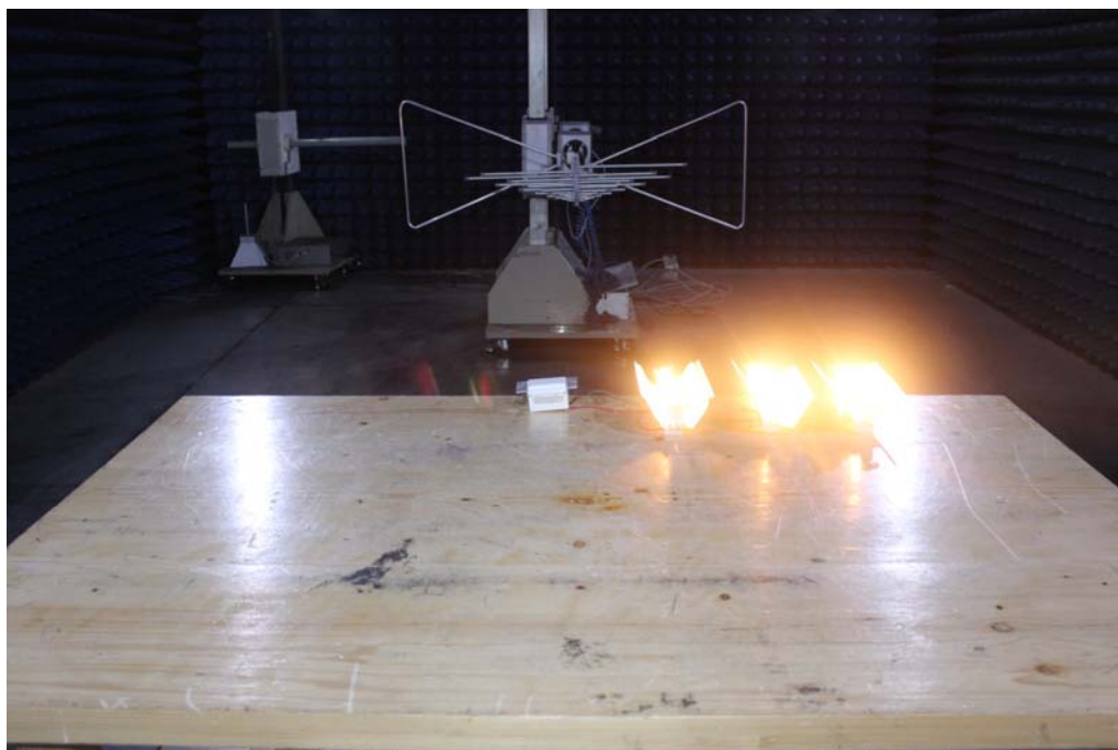
Photograph of set-up for Radiated Emission below 1GHz
