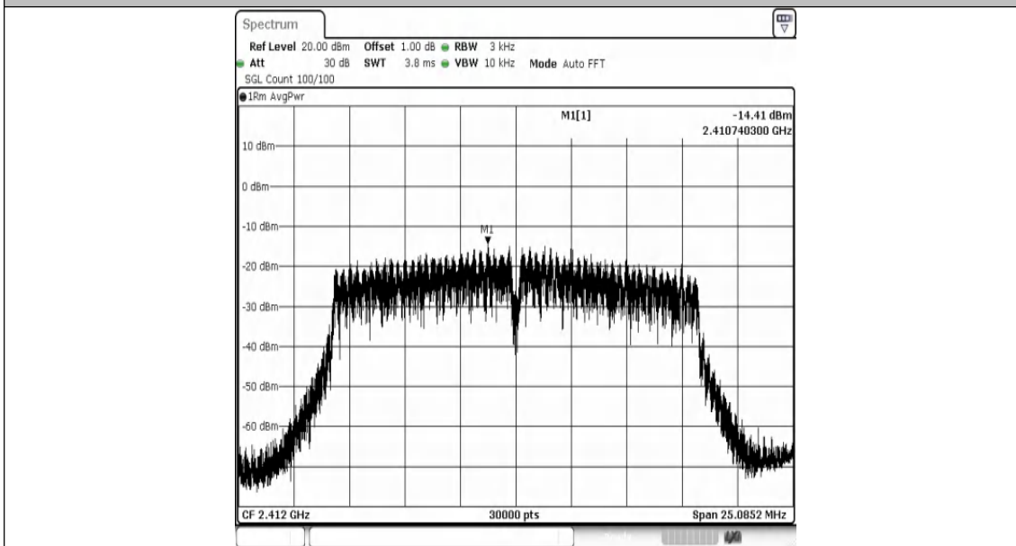
11G-Ant1-2412-PASS
