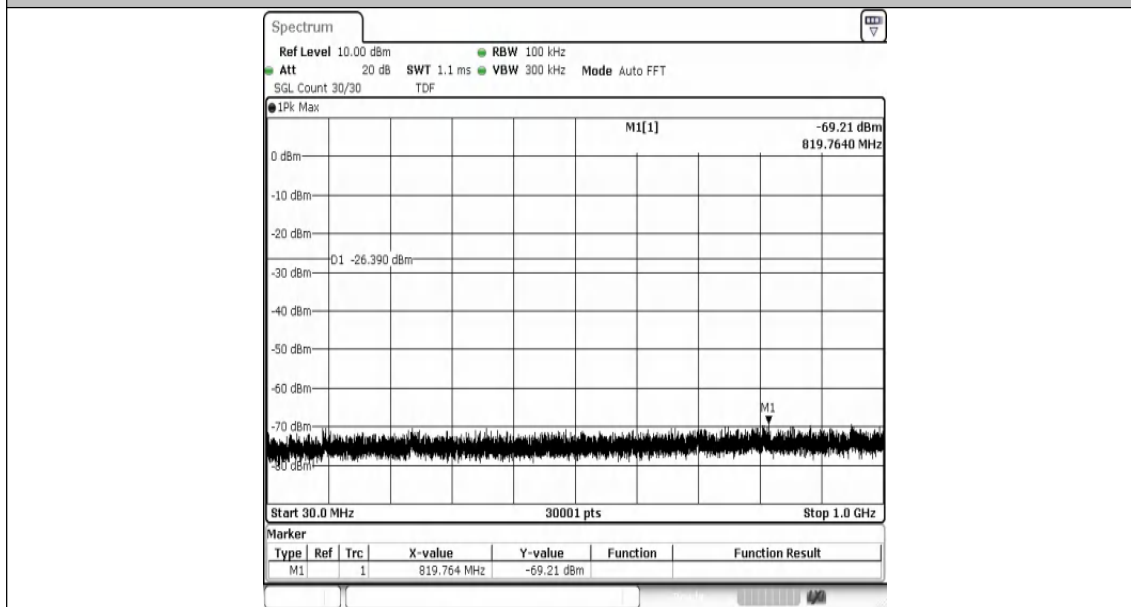
11N20SISO-Ant1-2412-30~1000-PASS
