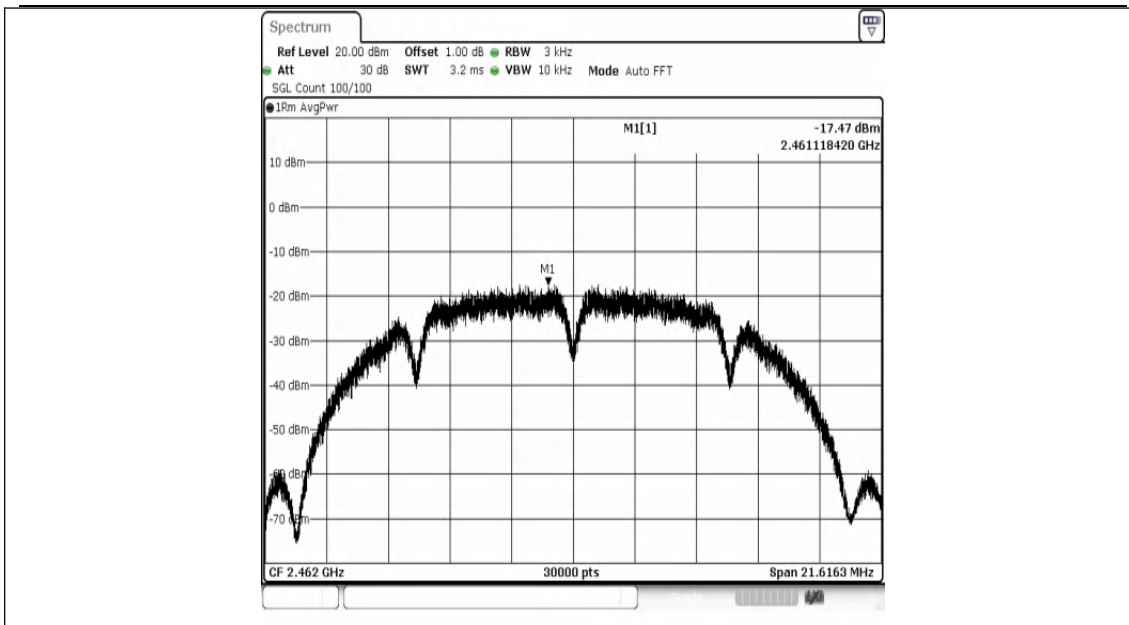
11B-Ant1-2462-PASS
