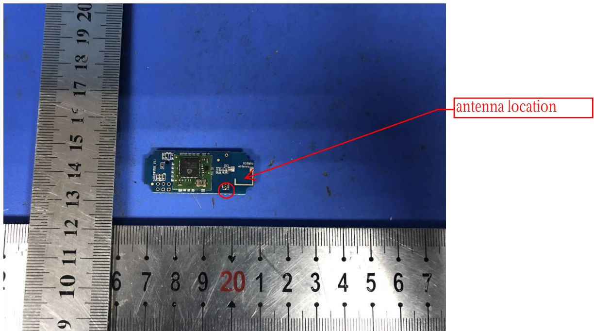
INTERNAL PHOTO OF SAMPLE – 6
