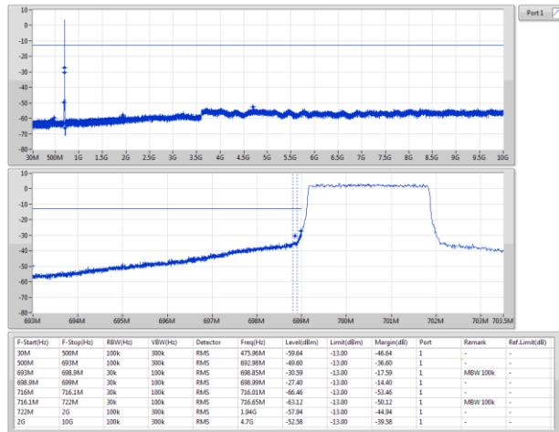
Band 12 LTE 3MHz_Nss1,16QAM_1TX 700.5MHz_16QAM_RB 1,#RB L
