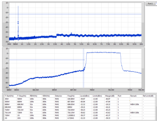
Band 12 LTE 5MHz_Nss1,16QAM_1TX 701.5MHz_16QAM_RB 1,#RB L
