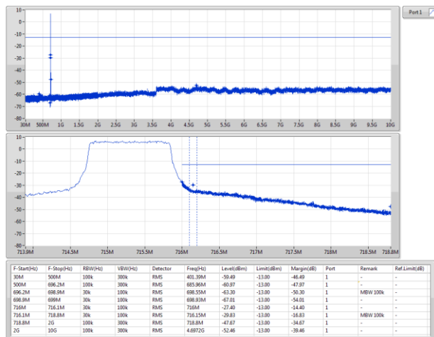
Band 12 LTE 1.4MHz Nss1,16QAM_1TX 715.3MHz_16QAM_RB 1,#RB H
