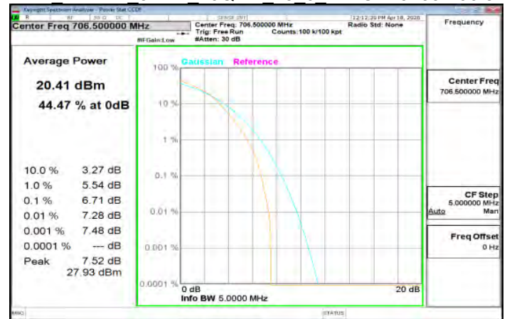
LTE Band17 5MHz 16QAM 25 0 LowCH23755-706.5
