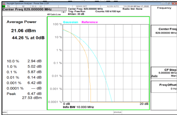
LTE Band5 10MHz 64QAM 50 0 LowCH20450-829
