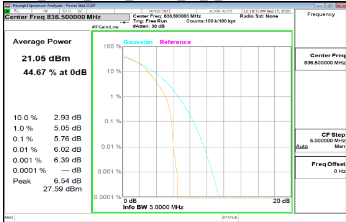
LTE Band5 3MHz 64QAM 15 0 MidCH20525-836.5
