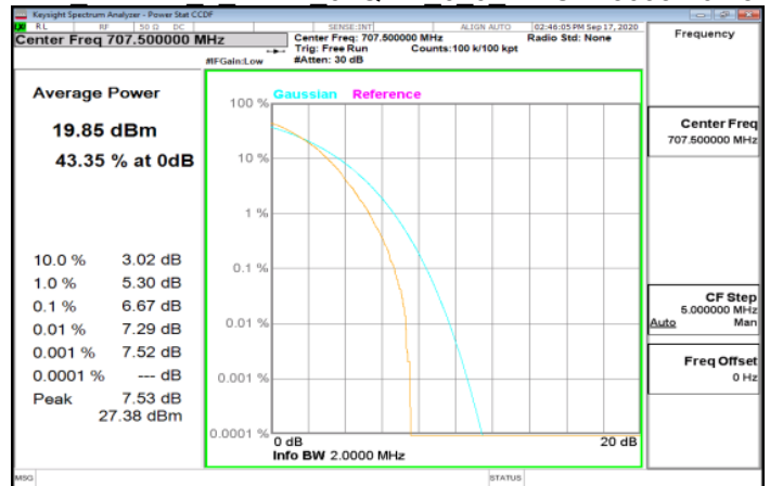
LTE Band12 1 4MHz 64QAM 6 0 MidCH23095-707.5
