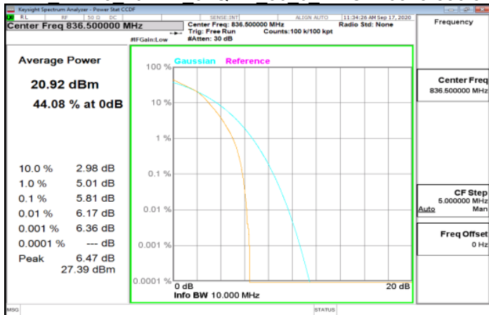
LTE Band5 10MHz 64QAM 50 0 MidCH20525-836.5
