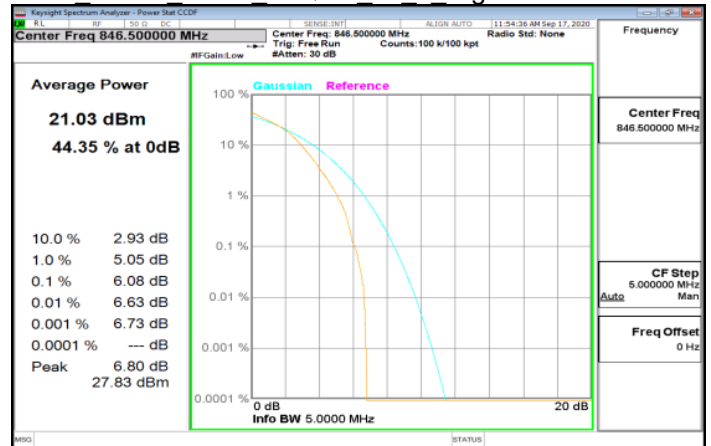
LTE Band5 5MHz 64QAM 25 0 HighCH20625-846.5
