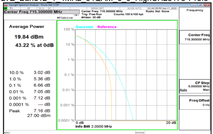
LTE Band12 1 4MHz 64QAM 6 0 HighCH23173-715.3
