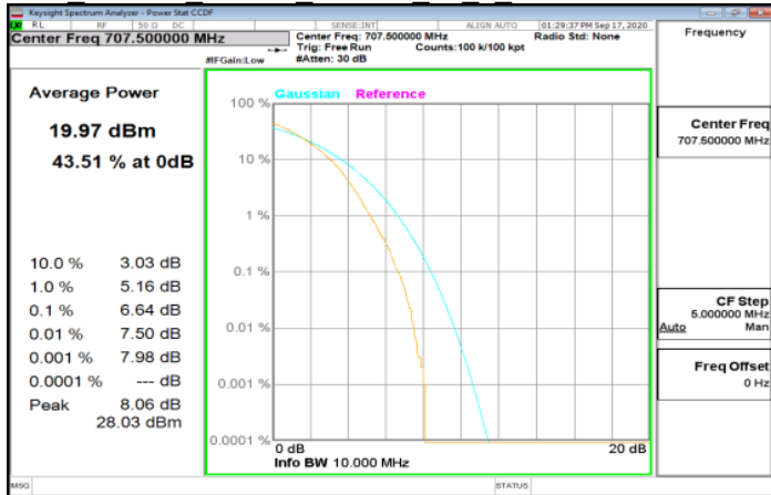
LTE Band12 10MHz 64QAM 50 0 MidCH23095-707.5
