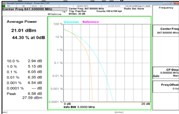
LTE Band5 3MHz 64QAM 15 0 HighCH20635-847.5
