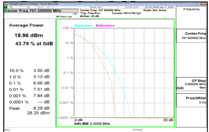
LTE Band12 5MHz 64QAM 25 0 MidCH23095-707.5
