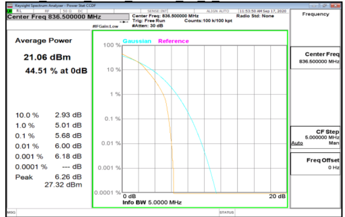
LTE Band5 5MHz 64QAM 25 0 MidCH20525-836.5
