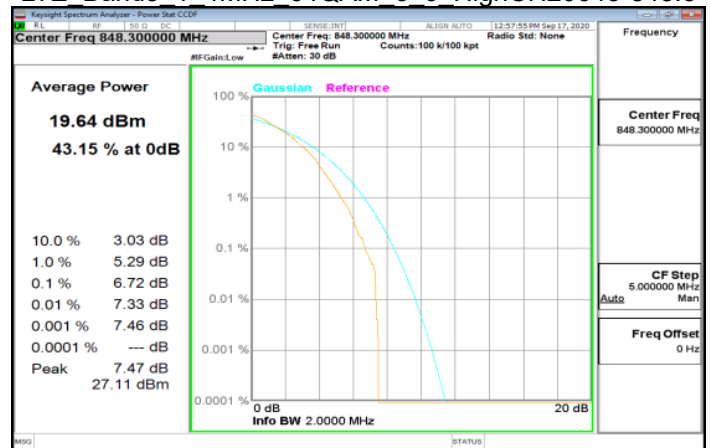
LTE Band5 1 4MHz 64QAM 6 0 HighCH20643-848.3
