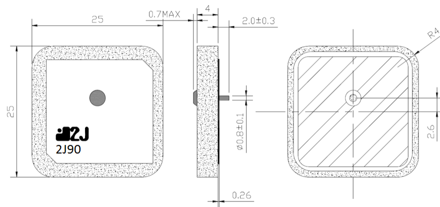
Patch dimensions
