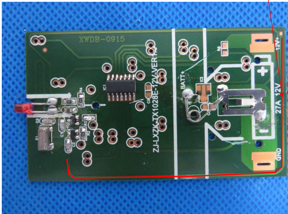
PCB Antenna
