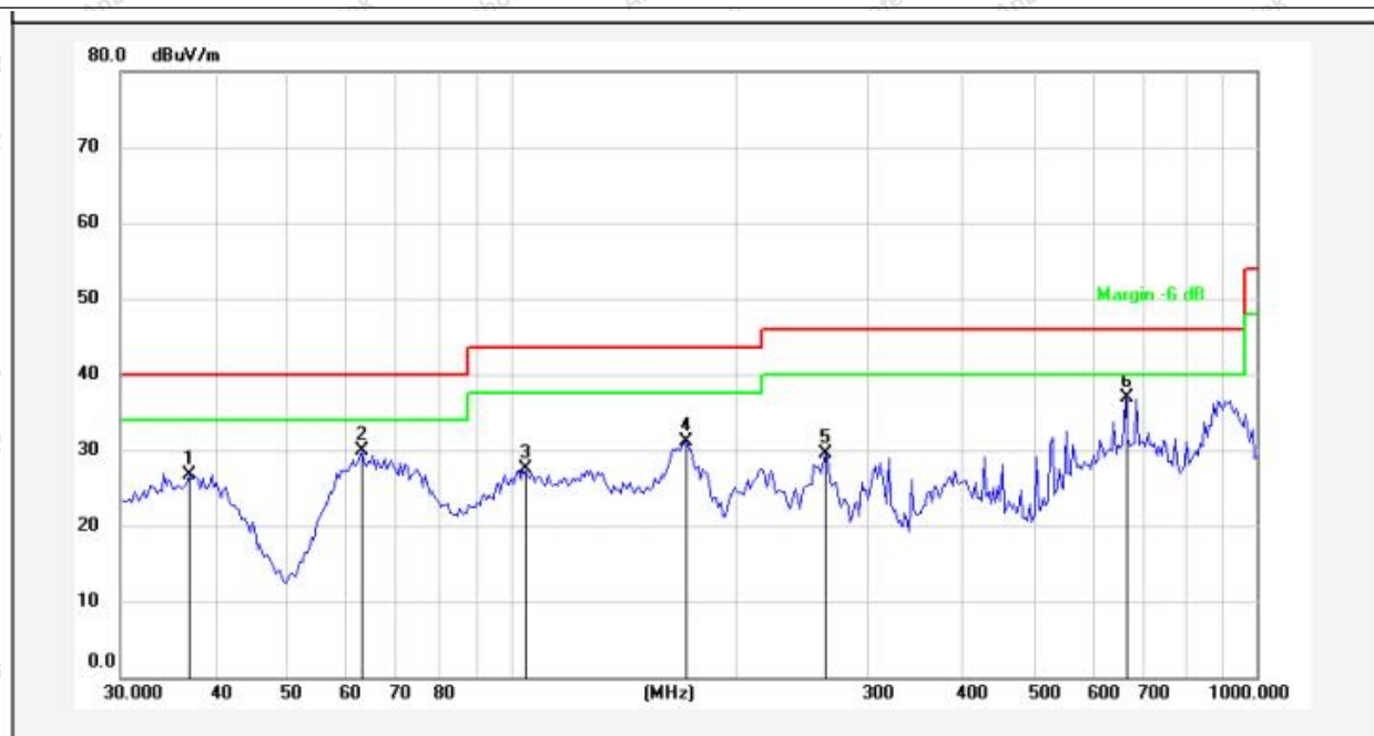
TM13 / Polarization: Horizontal
