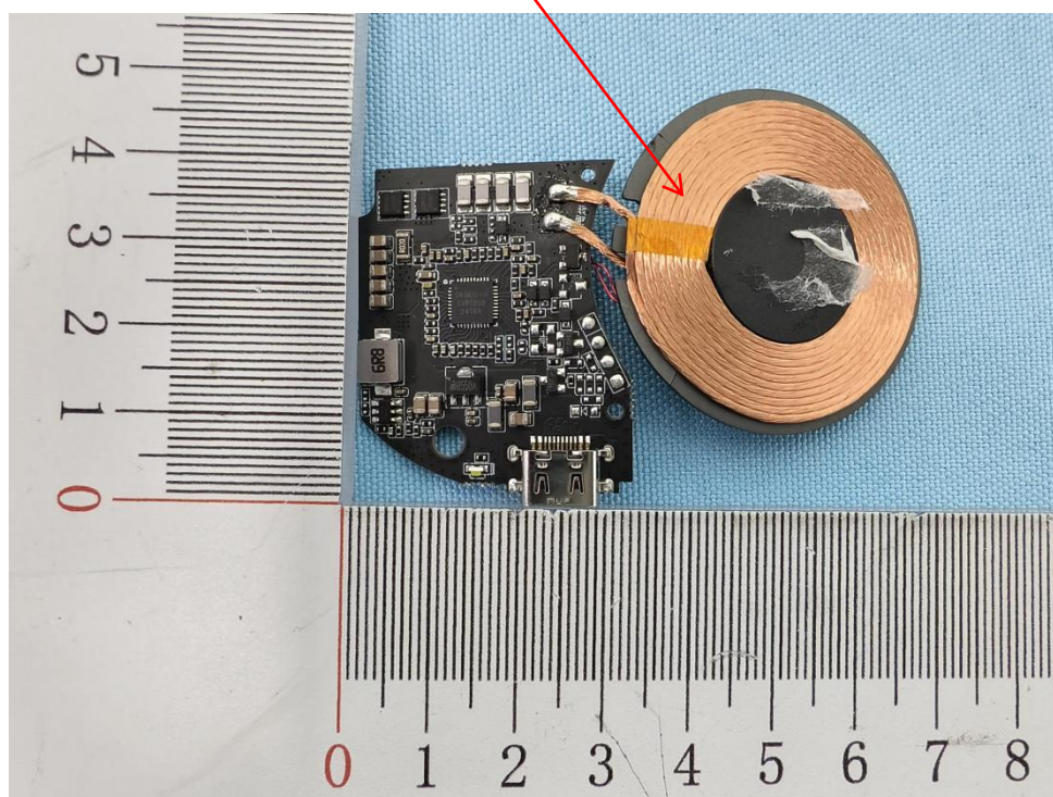
Earbuds-ANT
