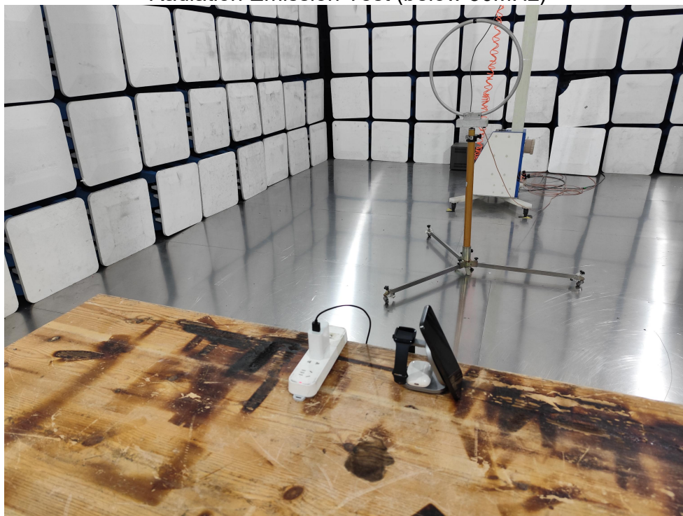
Radiation Emission Test (below 30MHz)
