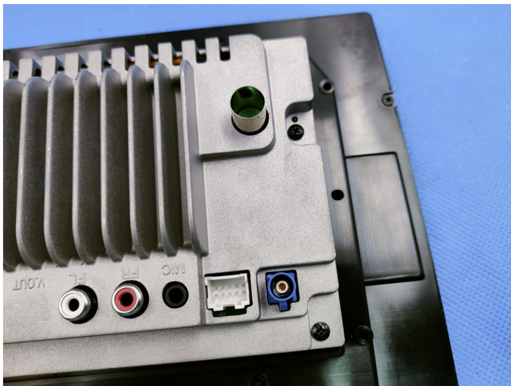
PORT VIEW OF EUT (FIGURE 3)
