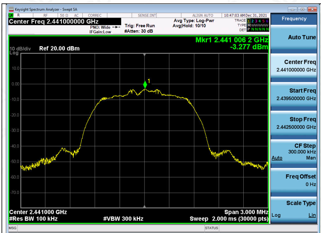
Test_Graph_EDR_ANT1_2441_2Mbps_Reference Level
