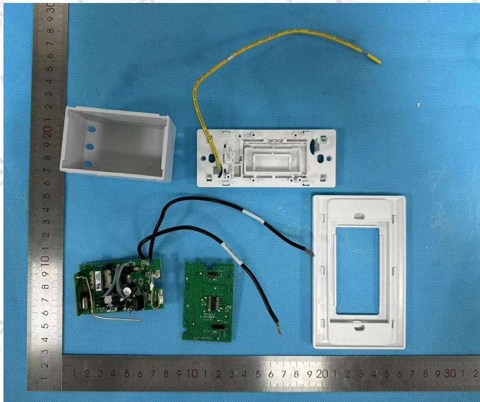
OPEN VIEW OF EUT(FIGURE 2)
