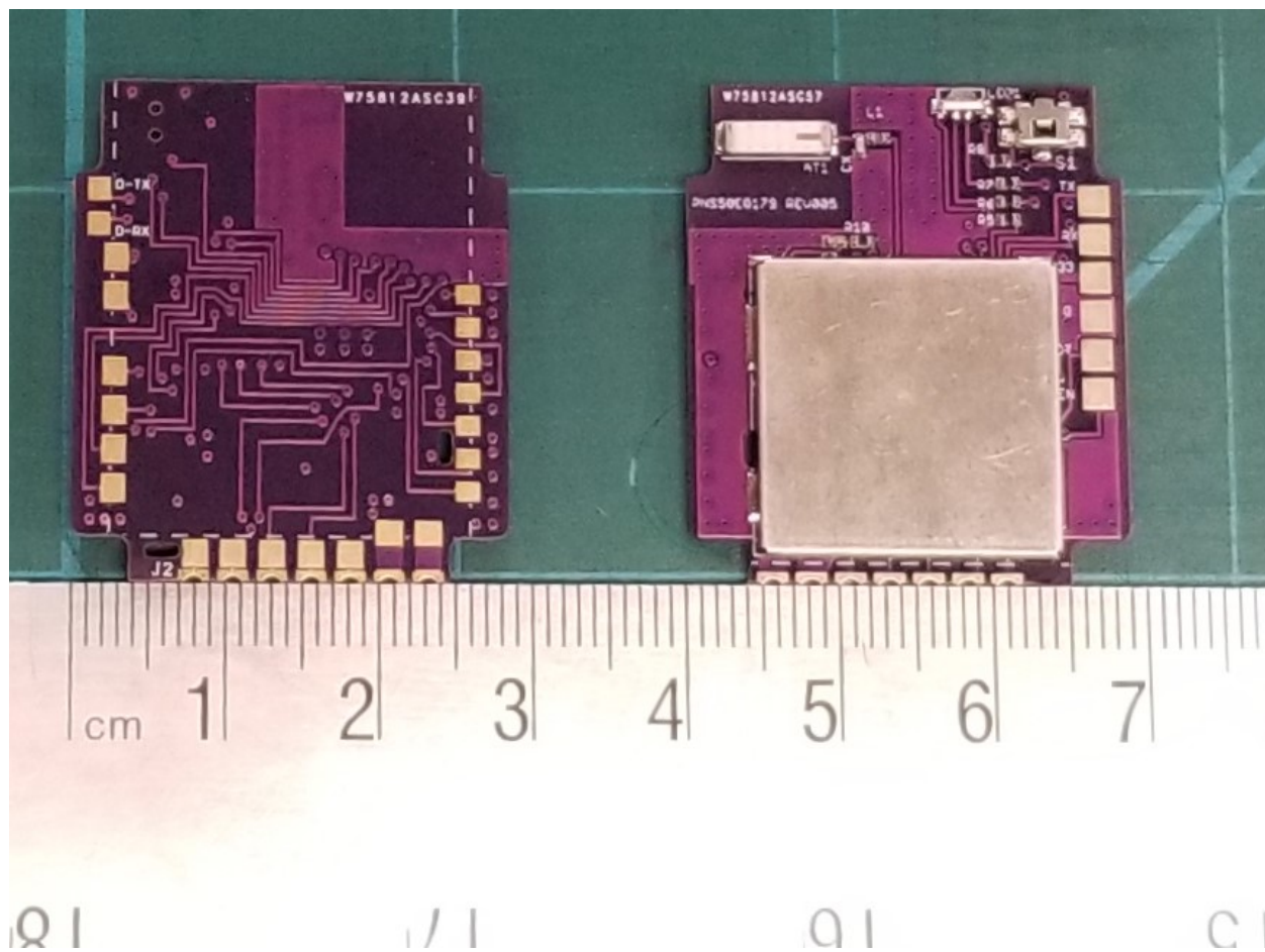
Figure 1: PCB Front/Back with Shield
