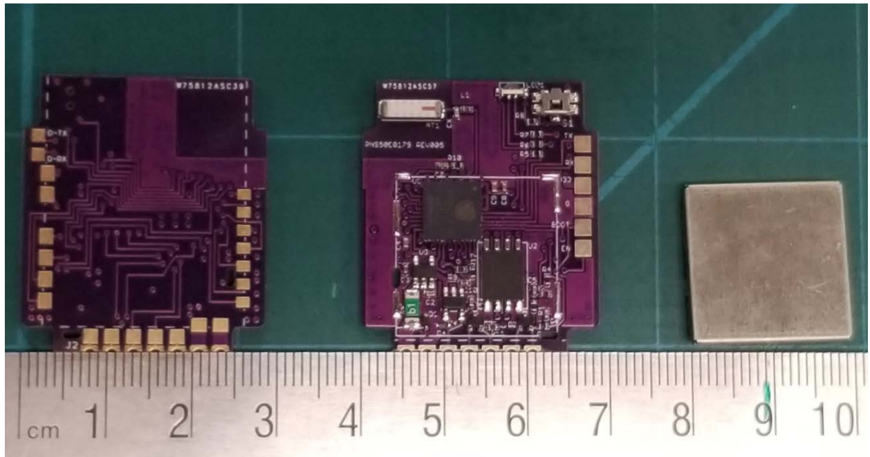
Figure 2: PCB Front/Back without Shield.
