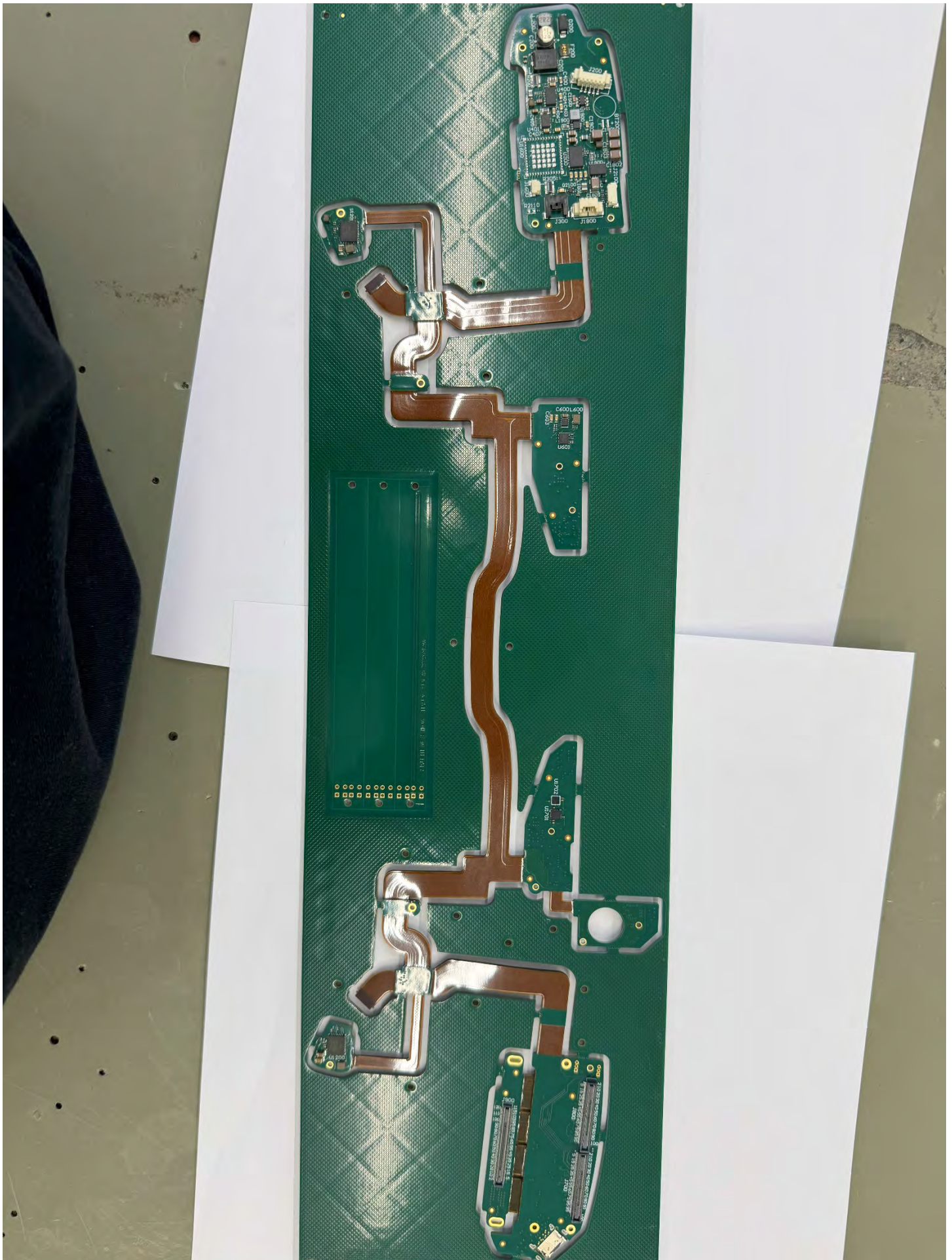
Main PCB Back Side Prior to Breakout for Assembly
