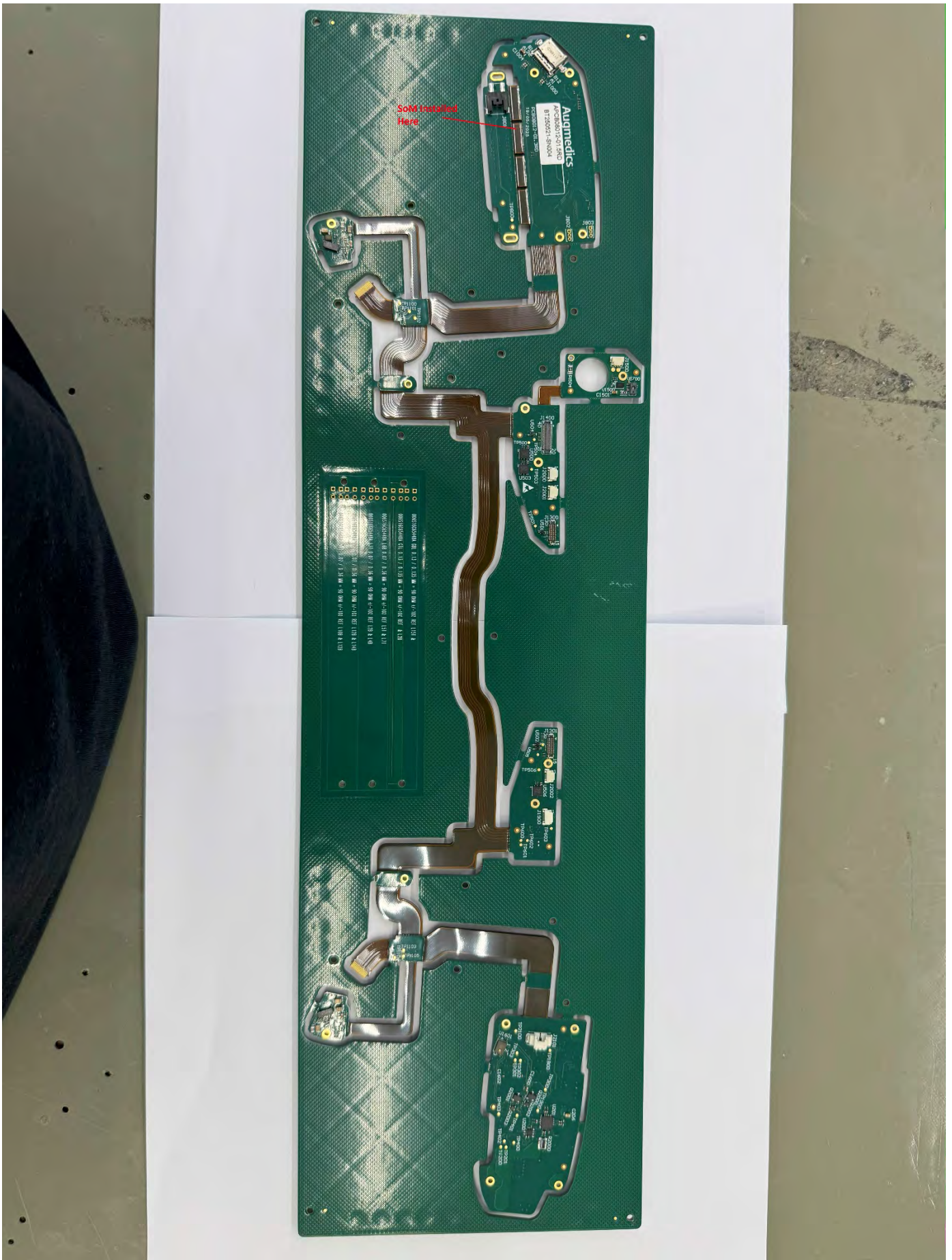
Main PCB Top Side Prior to Breakout for Assembly
