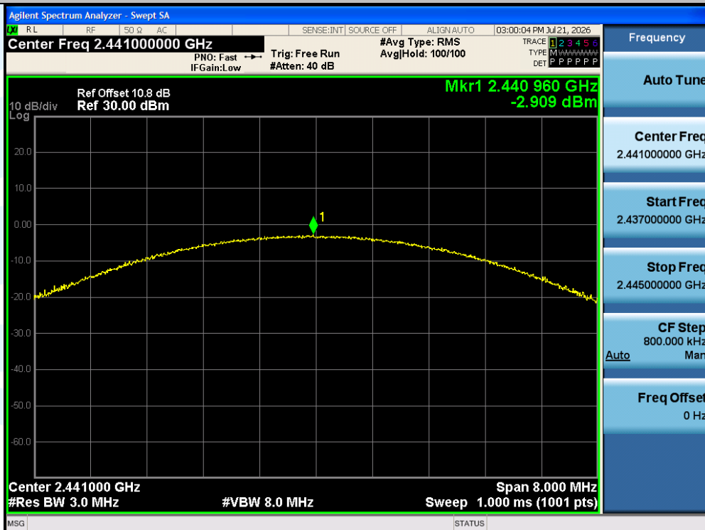
3DH5-Ant1-2441-PASS
