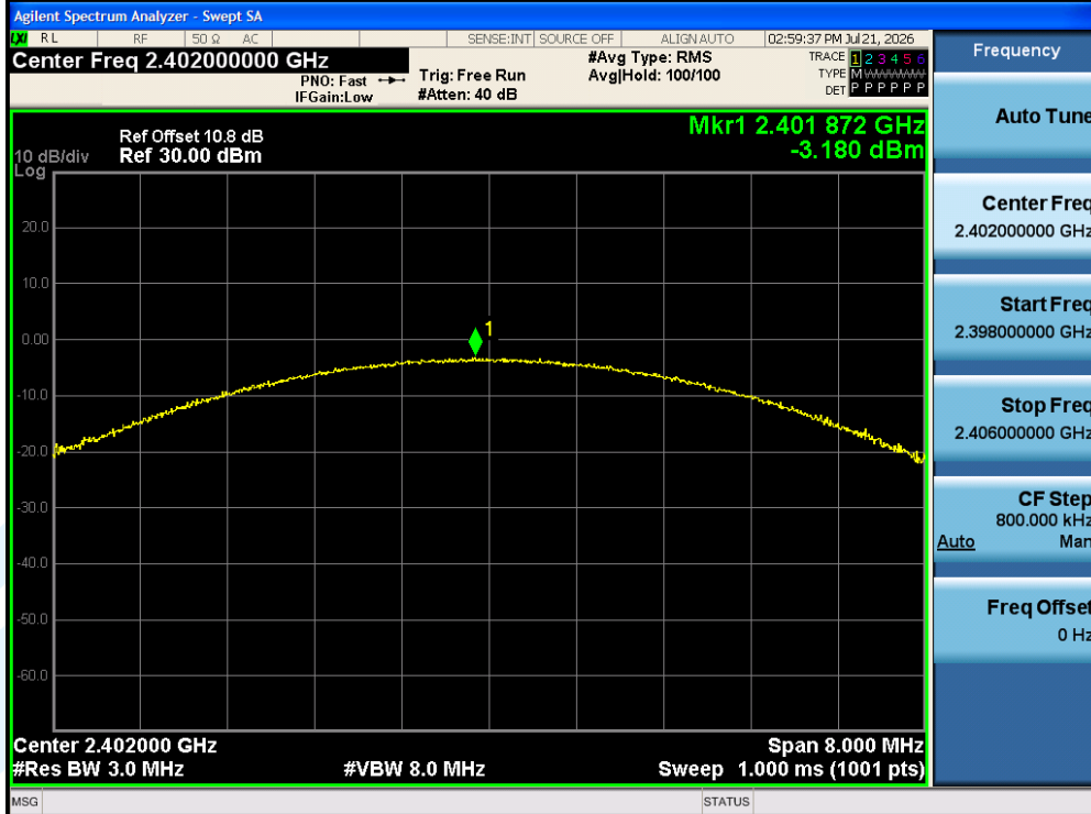
3DH5-Ant1-2402-PASS
