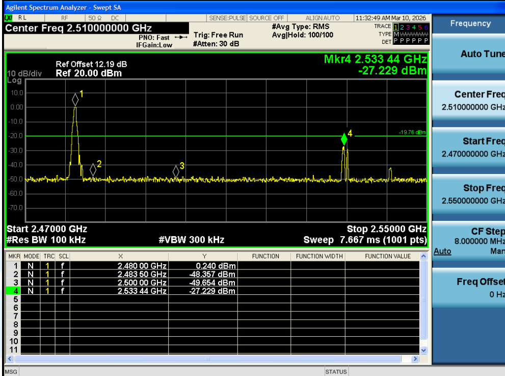
DH5-Ant1-2480-PASS
