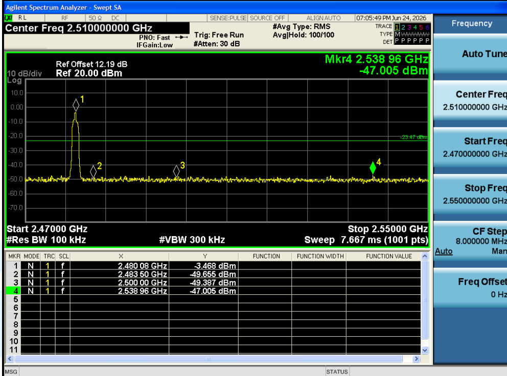
3DH5-Ant1-2480-PASS
