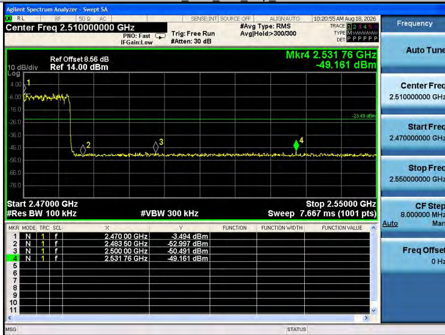
3DH5 Ant1 High Hop_2480
