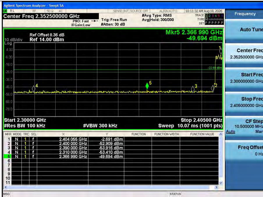
3DH5 Ant1 Low Hop_2402
