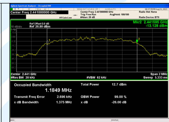
8DPSK_3-DH5_Channel 39
