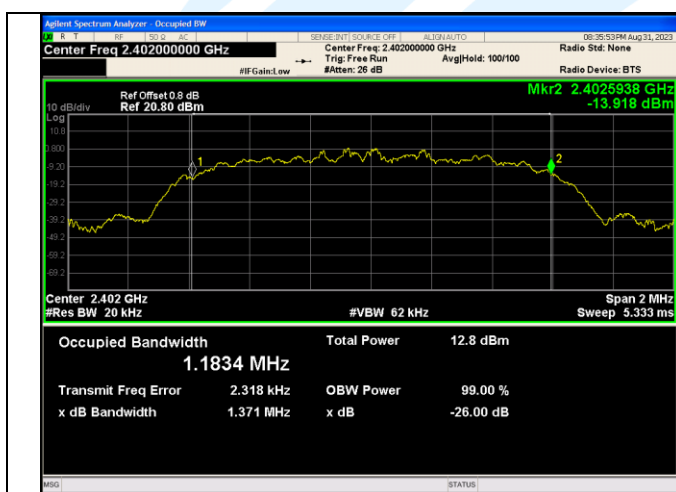
8DPSK_3-DH5_Channel 0
