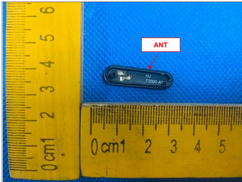
Left earphone
