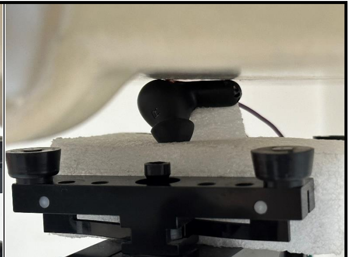
Test Position 2 (EUT with 0 cm Gap)
