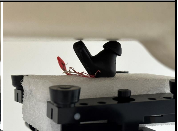
Test Position 4 (EUT with 0 cm Gap)
