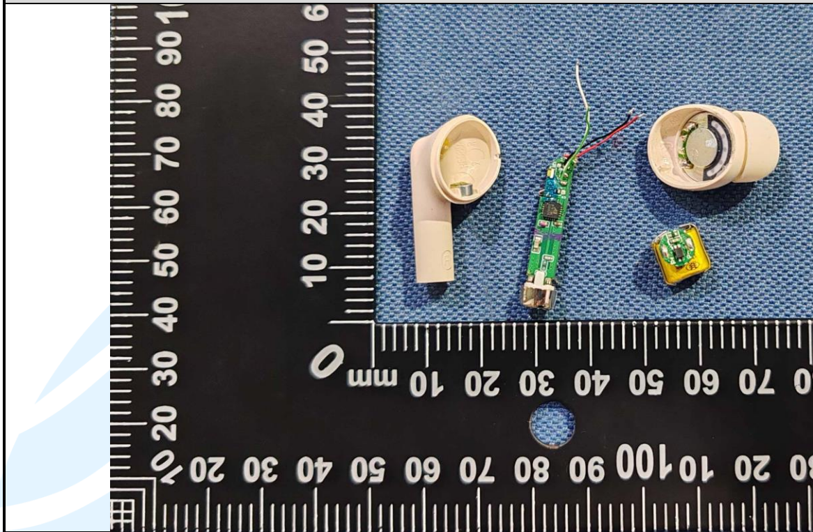
EUT Photo(Right earbud)
