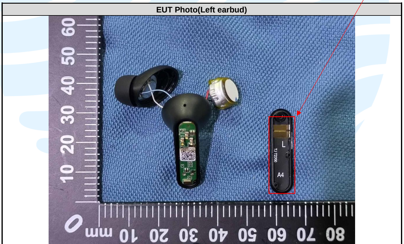
EUT Photo(Left earbud)
