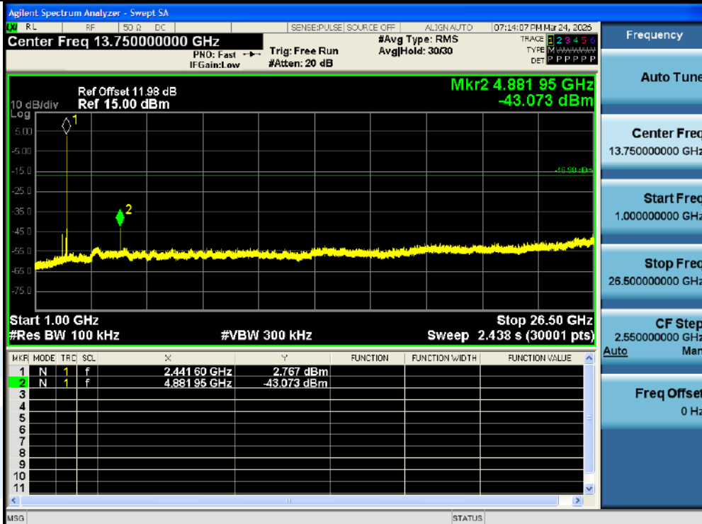
DH5-Ant1-2441-1000~26500-PASS
