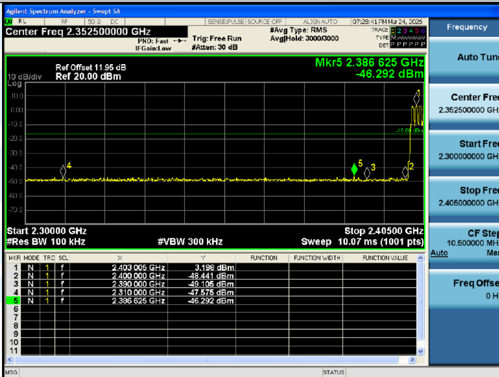
DH5-Ant1-Hop_2402-PASS
