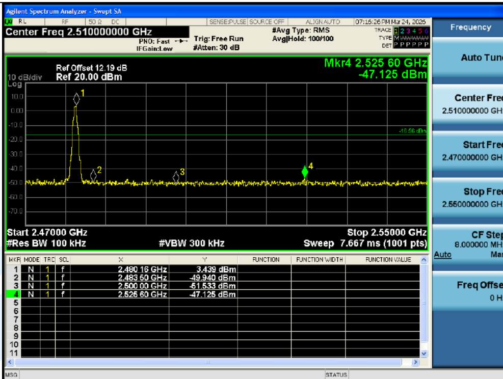
DH5-Ant1-2480-PASS
