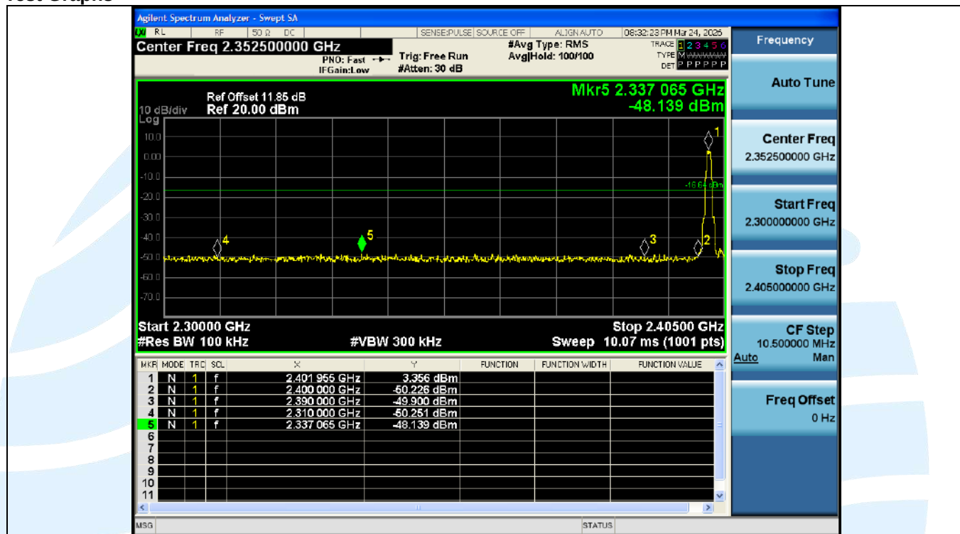
BLE_1M-Ant1-2402-PASS
