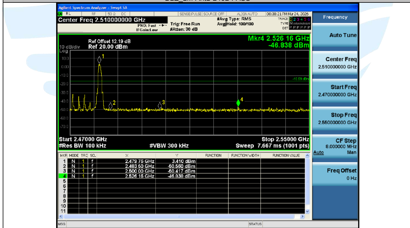
BLE_1M-Ant1-2480-PASS
