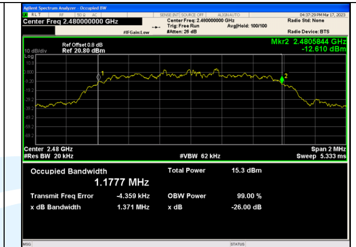
\pi/4 DQPSK_2-DH5_Channel 78
