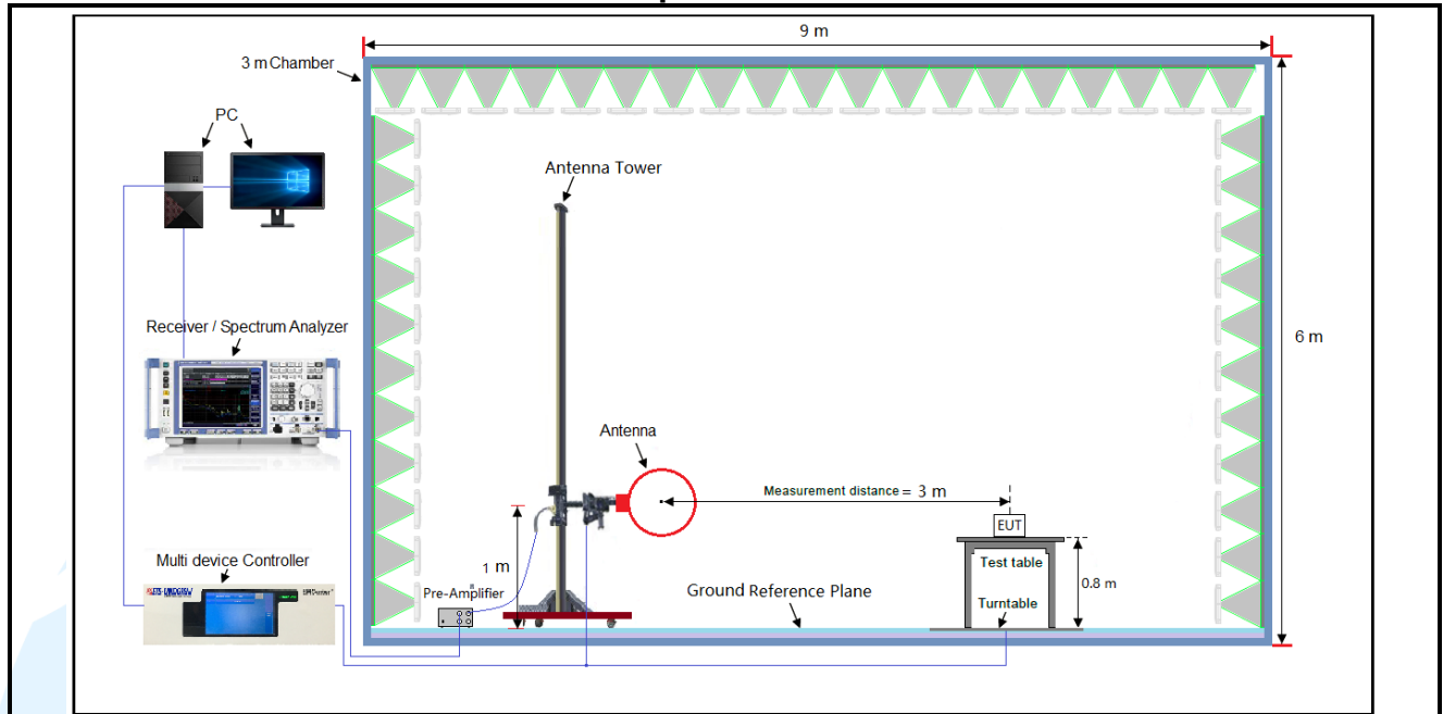
Figure 1. Below 30MHz
