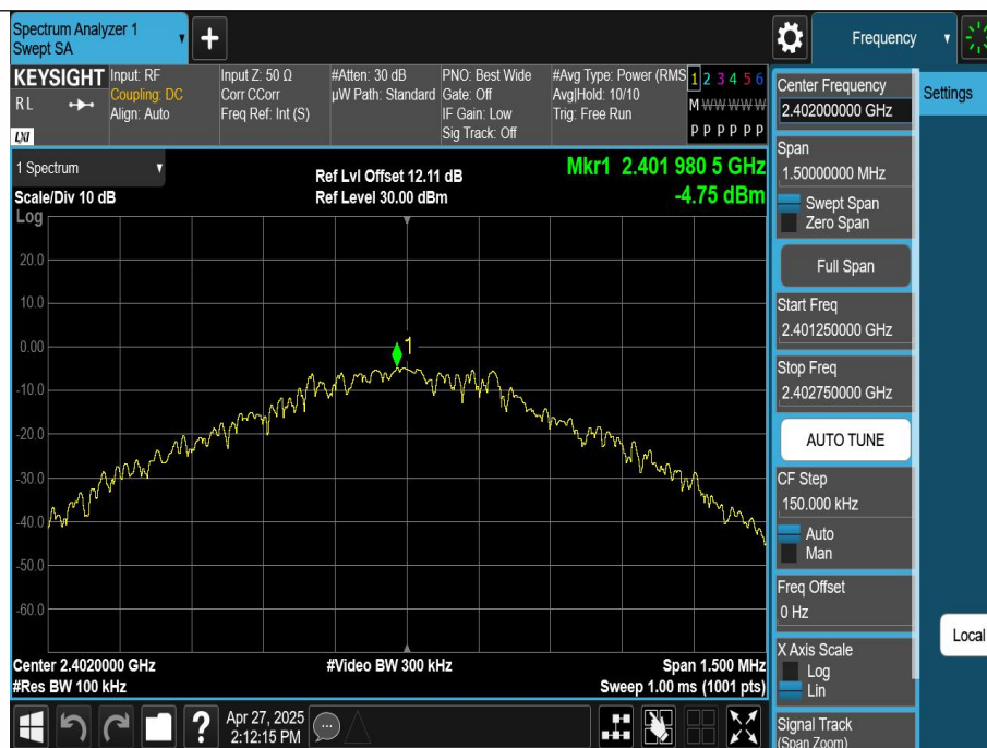
DH5-Ant1-2402-0~Reference-PASS
