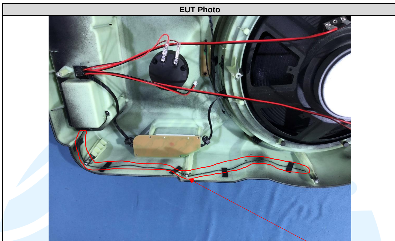
FM Antenna (only receive)
