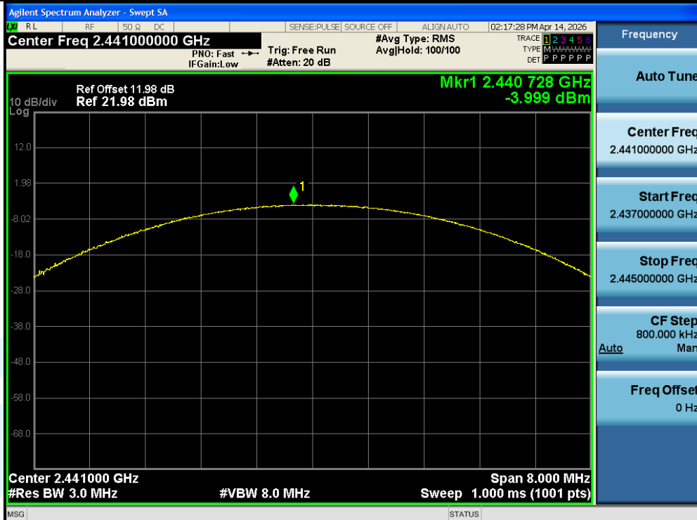
2DH5-Ant1-2441-PASS
