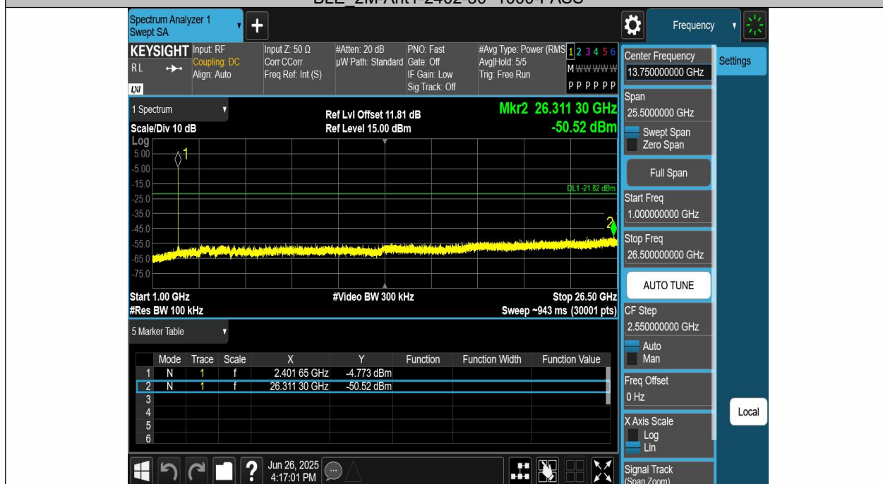
BLE_2M-Ant1-2402-1000~26500-PASS
