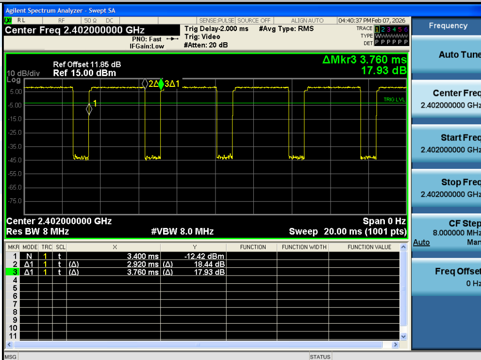
NTNV-3DH5-Ant1-2402
