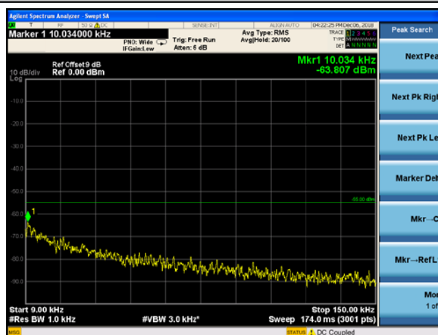
Band7_5MHz_QPSK_21100_1RB#0
