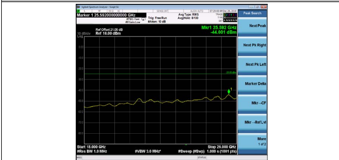
Band7_10MHz_16QAM_21100_1RB#0
